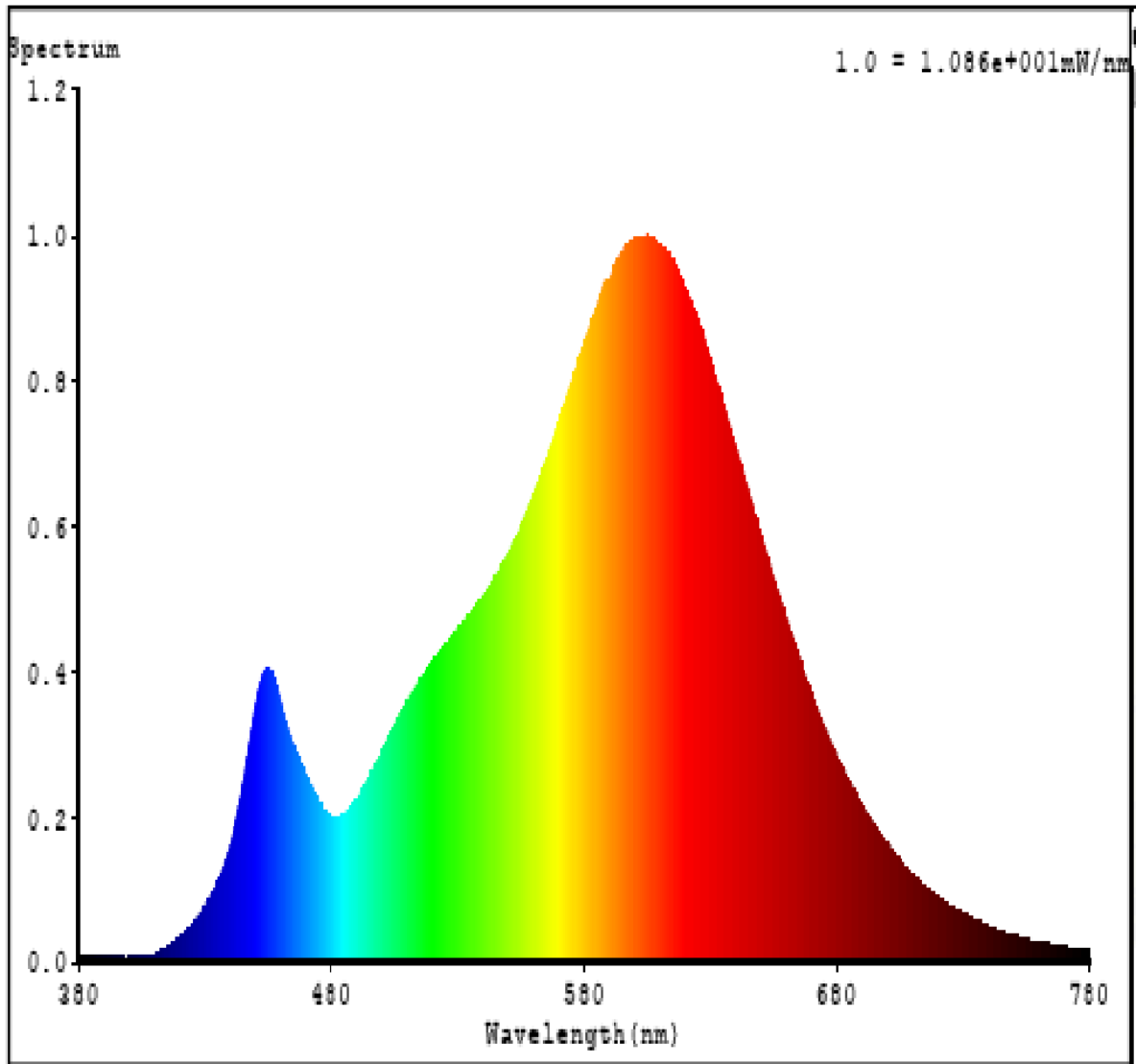
Spectral Distribution
