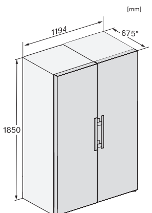
KS4783ED N, KS4784ED N, KS4885DD N, FNS4782E N, FNS4882D, Nordic, installation sketch, Side-by-Side
