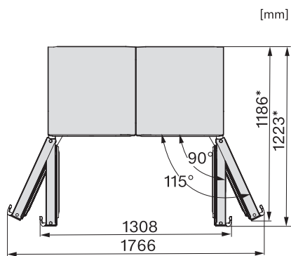
FNS4383E N, FNS4782E N, FNS4782D N, FNS4882D N, FNS4383D N, Nordic, installation
